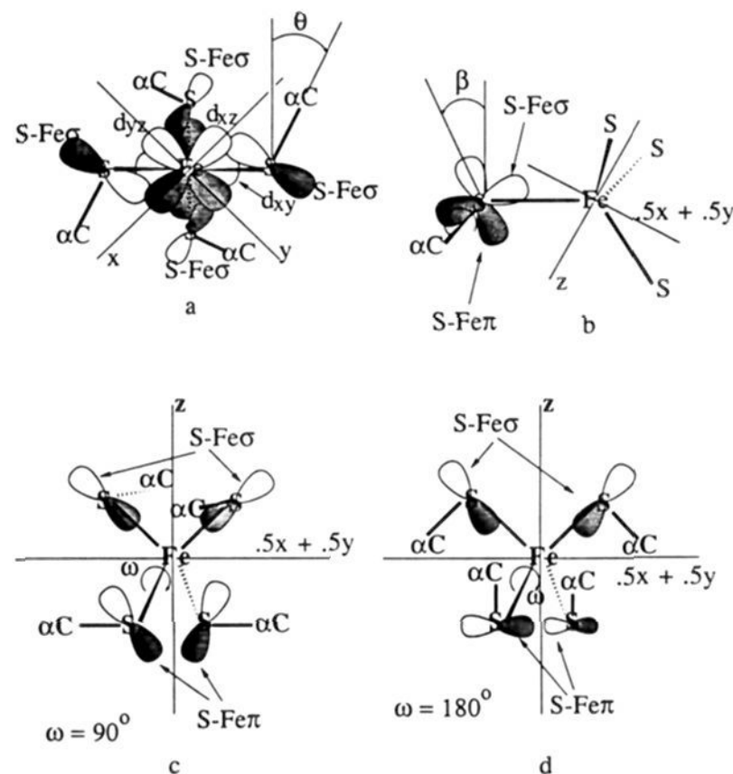
Figure 15. (a) View down the molecular z axis showing the effect of the \alpha\text{C} bond angle ( >90^\circ ) on the orientation of the \text{S-Fe}\sigma orbital relative to the \text{Fe } d_{xz,yz} and d_{xy} orbitals. (b) View down one of the \alpha\text{C-S} bonds showing the effect of the rotation ( \beta ) on the orientations of the \text{S-Fe}\sigma and \text{S-Fe}\pi orbitals relative to the iron center. (c) View perpendicular to the molecular z axis showing the orientations of the \text{S-Fe}\sigma and \text{S-Fe}\pi orbitals relative to the iron center when \omega = 90^\circ . (d) View perpendicular to the molecular z axis showing the orientations of the \text{S-Fe}\sigma and \text{S-Fe}\pi orbitals relative to the iron center when \omega = 180^\circ .
