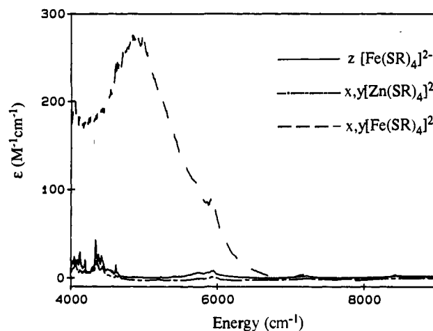
Figure 5. Polarized absorption spectra at 7 K for a 100 \mu\text{m} thick [\text{N}(\text{Et})_2][\text{Zn}(\text{Fe})\text{-(SR)}_4] ( [\text{Fe}] = 30\% ) crystal taken on the (010) face and a 225 \mu\text{m} thick [\text{N}(\text{Et})_2][\text{Zn}(\text{SR})_4] crystal taken on the (001) face.
