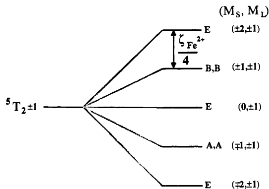
Figure 12. In-state spin-orbit splitting of the ligand-field 5 T 2 (±1) state, showing the transformation properties in S 4 symmetry of the doublets. Also shown is the spin and orbital wave functions which comprise each state.
