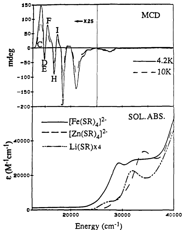
Figure 9. (Top) Single-crystal MCD spectrum at 50 kG for a 100 \mu\text{m} thick [\text{N}(\text{Et})_4]_2[\text{Zn}(\text{Fe})-(\text{SR})_4] ( [\text{Fe}] = 0.2\% ) crystal taken on the (001) face. The MCD features below 25 000 \text{cm}^{-1} have been multiplied by 25. (Bottom) Room temperature solution absorption spectra for [\text{Fe}(\text{SR})_4]^{2-} , [\text{Zn}(\text{SR})_4]^{2-} , and LiSR. The LiSR spectra has been multiplied by four.
